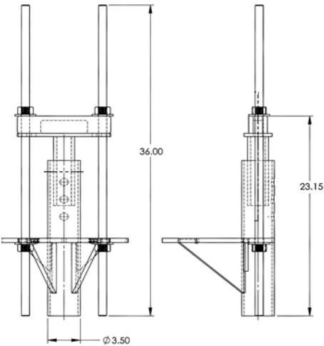
FIGURE 2—TRU-LIFT BRACKET (TLB)
