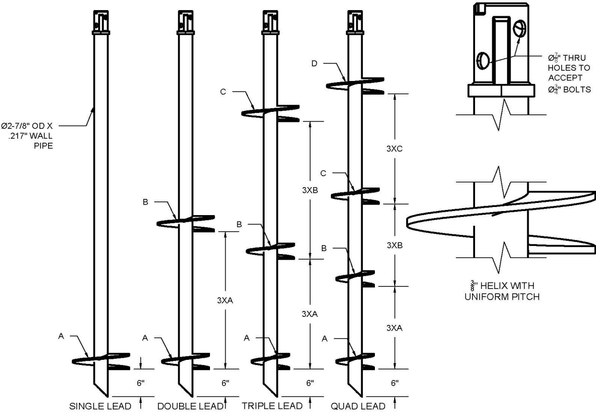
FIGURE 3—HELICAL LEAD SHAFTS
